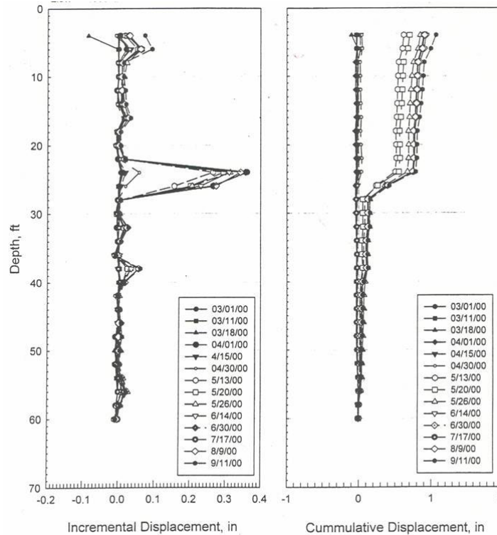
Figure 6-3. Concentrated Movements Recorded from Inclinator at the Slip Surface (after Liang, 2000).
